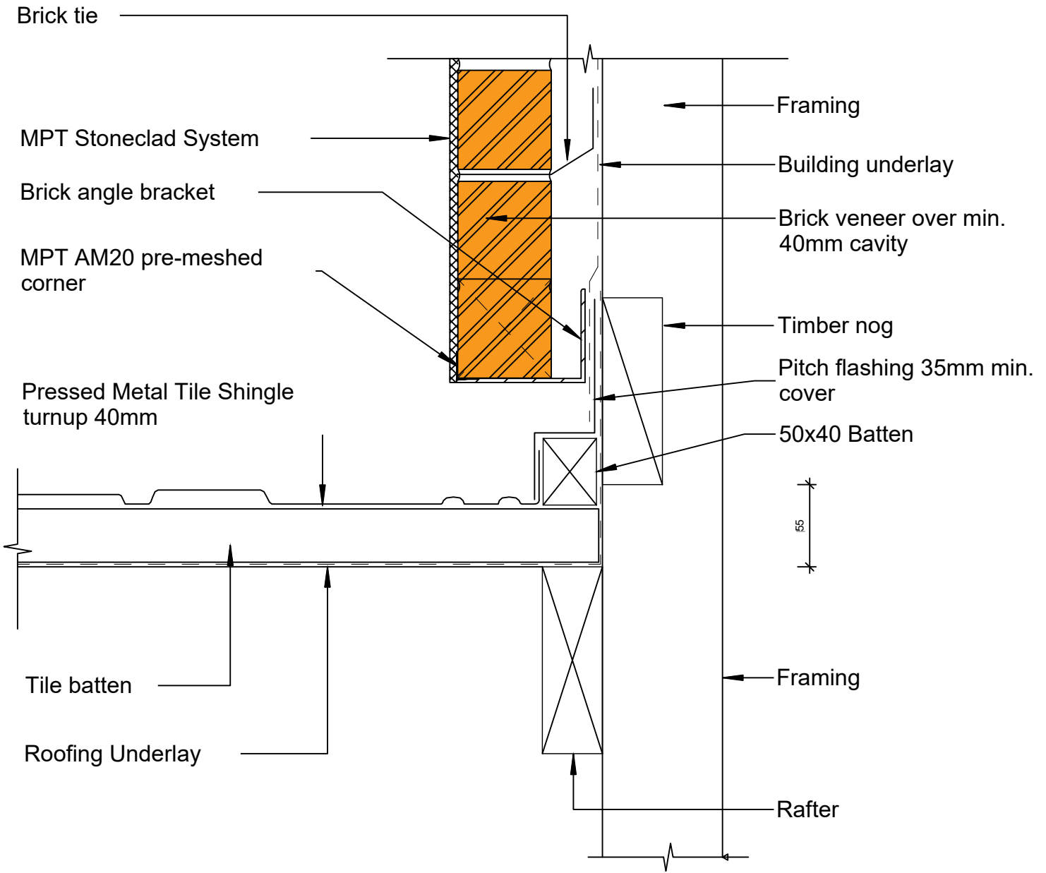
Roof installed before Brick Veneer cladding installed
